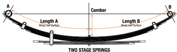
TWO STAGE SPRINGS
