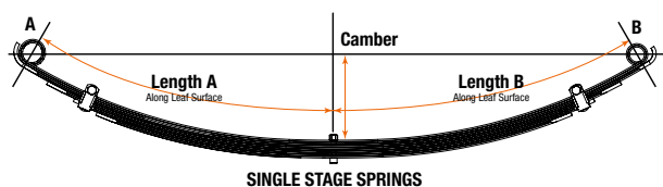
SINGLE STAGE SPRINGS
